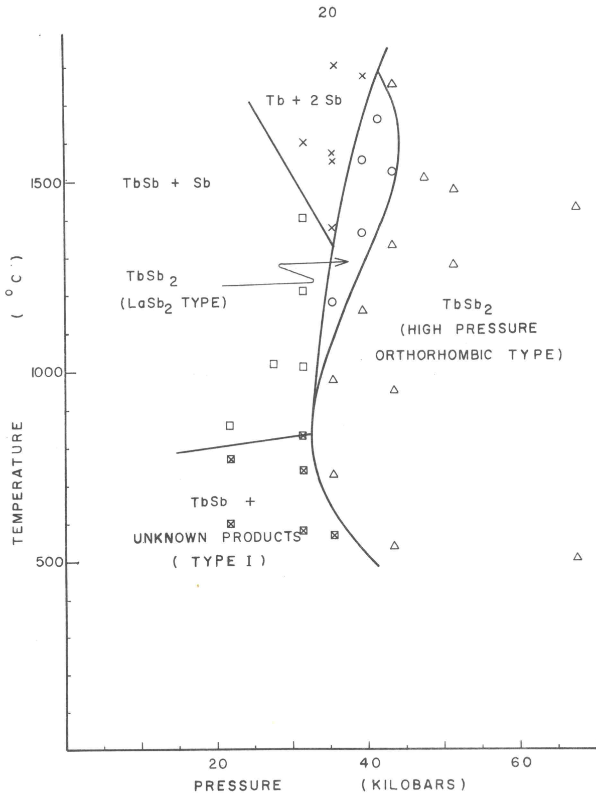
Fig. 6.--Tb + 2 Sb Reaction Product Diagram.
